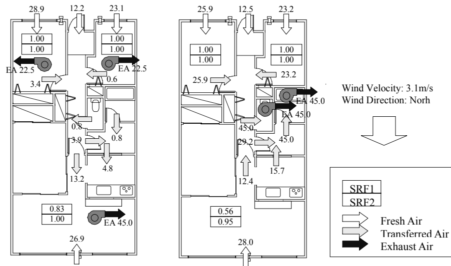
Airflow rate and performance of mechanical ventilation in flat
