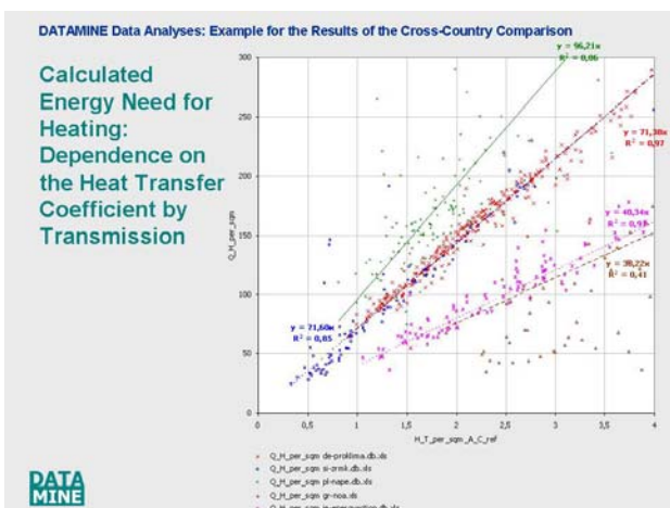
Figure 11. Analyses of the energy performance calculated by the respective national EPC procedures and comparison between different countries / regions.
