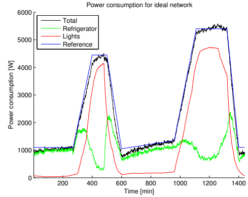
Fig. 8: Base case simulation of the controller under ideal network conditions.
