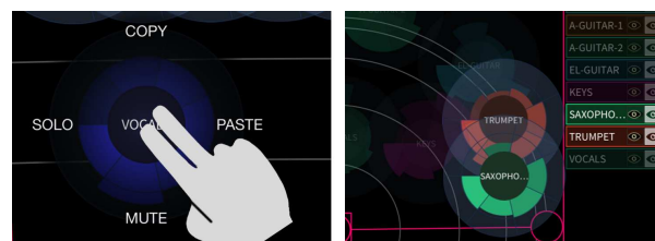
Fig. 4: Left: Touching the widget with two fingers brings up a menu providing additional settings. The user then moves up, down, right or left and releases to select the menu point. Right: Visual layers provide ability to show/hide certain widgets.
