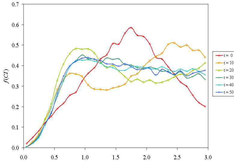
Figure 8. Density function of condition index CI for minor concrete repair strategy based on 50,000 simulations.
