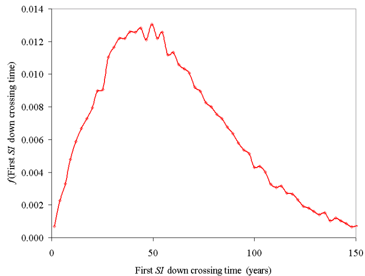
Figure 11. Density function of first SI downcrossing time for minor concrete repair strategy based on 50,000
