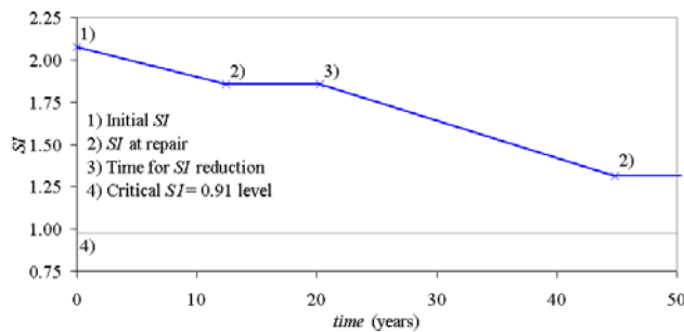
Figure 3. A realization of the safety index SI for a minor concrete repair strategy.
