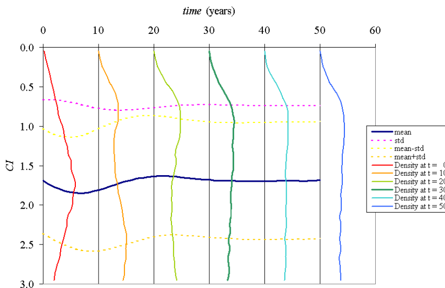
Figure 5. The condition index CI for the minor concrete repair strategy based on 50 000 simulations. Density functions are multiplied by a factor
