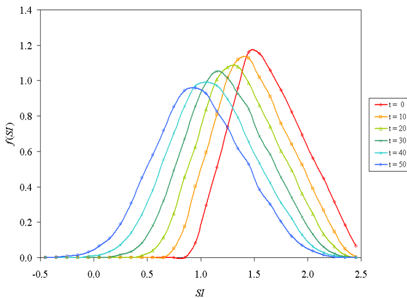
Figure 9. Density function of safety index for minor concrete repair strategy based on 50,000 simulations.
