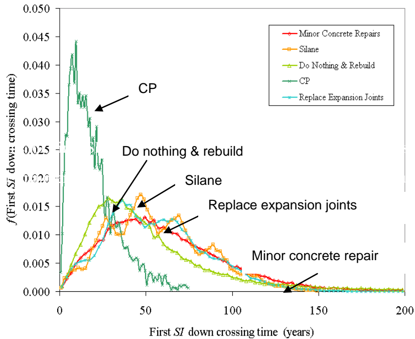
Figure 12. Comparison of first safety index SI downcrossing distributions (for CP strategy, only 3,535 realizations (7.07 %) had finite downcrossing).
