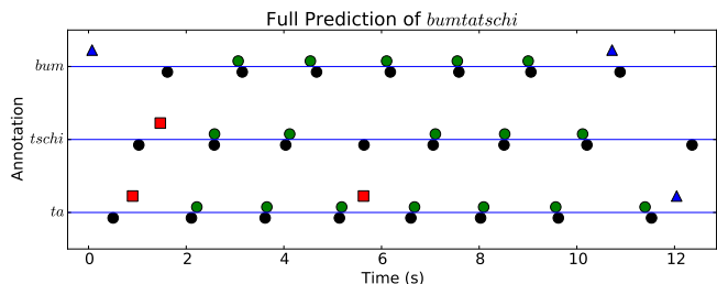
Fig. 7. The system (with HN) quickly captures a simple ta-tschi-bum pattern. Time (horizontal axis) is mapped versus event labels (one line each for 'ta', 'tschi', and 'bum'). Annotated labels are indicated in black below the lines. Above the horizontal lines we find events that are correctly estimated ('●'), matched to the wrong cluster ('■'), and unmatched ('▲') due to a wrongly estimated onset.
