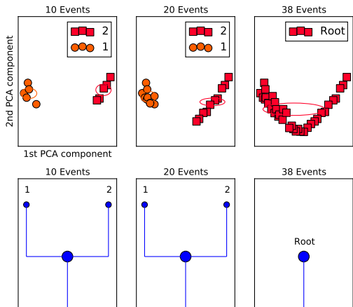
Fig. 9. Cluster merging: After 38 events, two clusters ('●', '■') merge into one cluster ('■'). The projection of the MFCC vectors (timbre representation) onto their first two principal components ( above ) and the incremental clustering tree ( below ) are shown.
