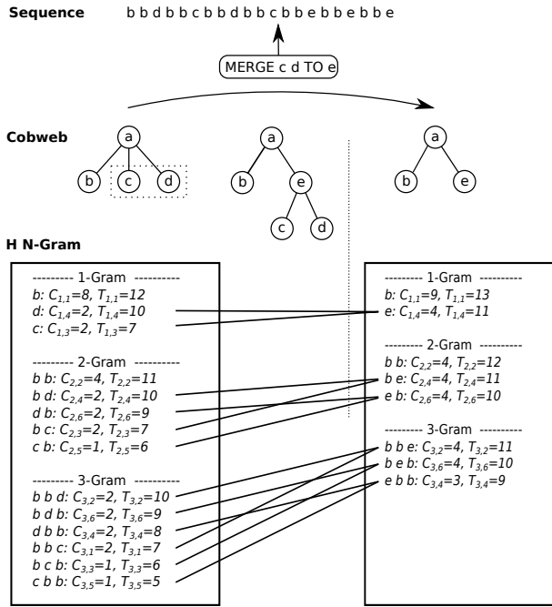
Fig. 2. The Effect of a concept merge in the hierarchical n-gram. Nodes c and d are merged into the new symbol e . The n -gram inherits the counts for patterns including c and d to patterns including e .
