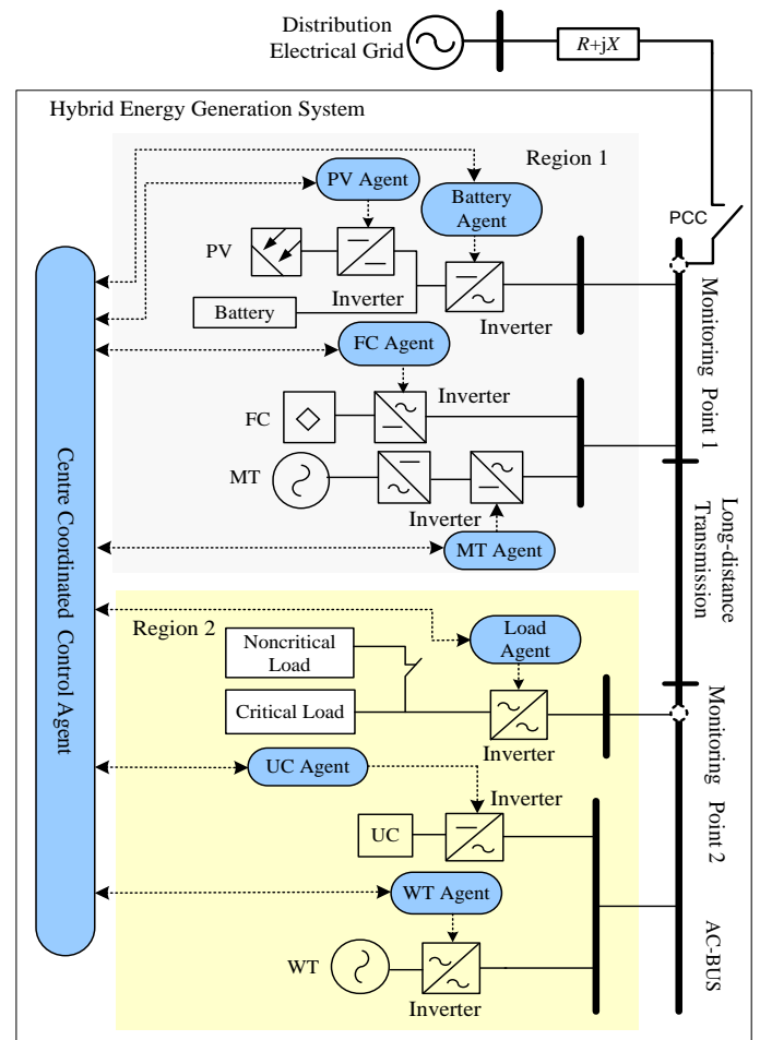
Fig. 1. MAS based control scheme of HEGS.
