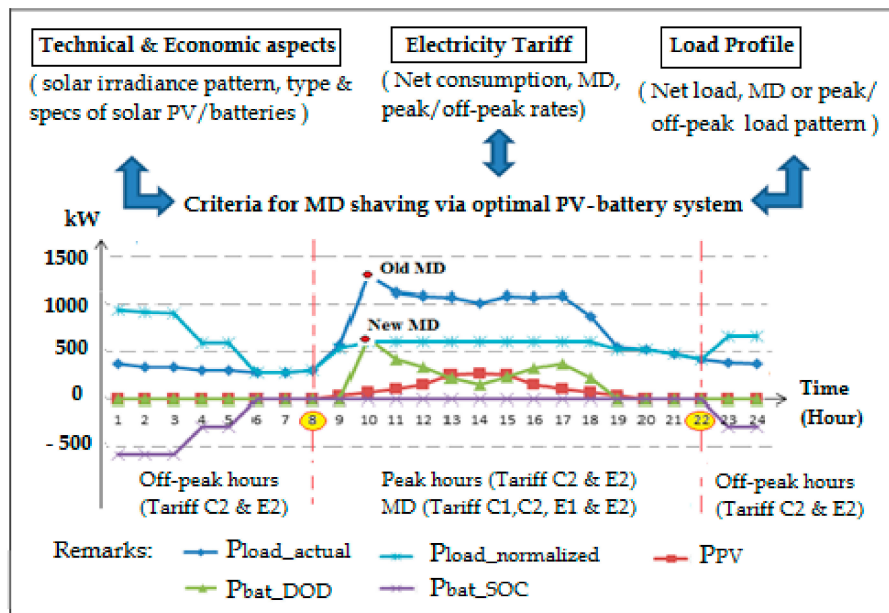
Figure 7. Criteria for maximum demand (MD) shaving optimal PV-battery system.
