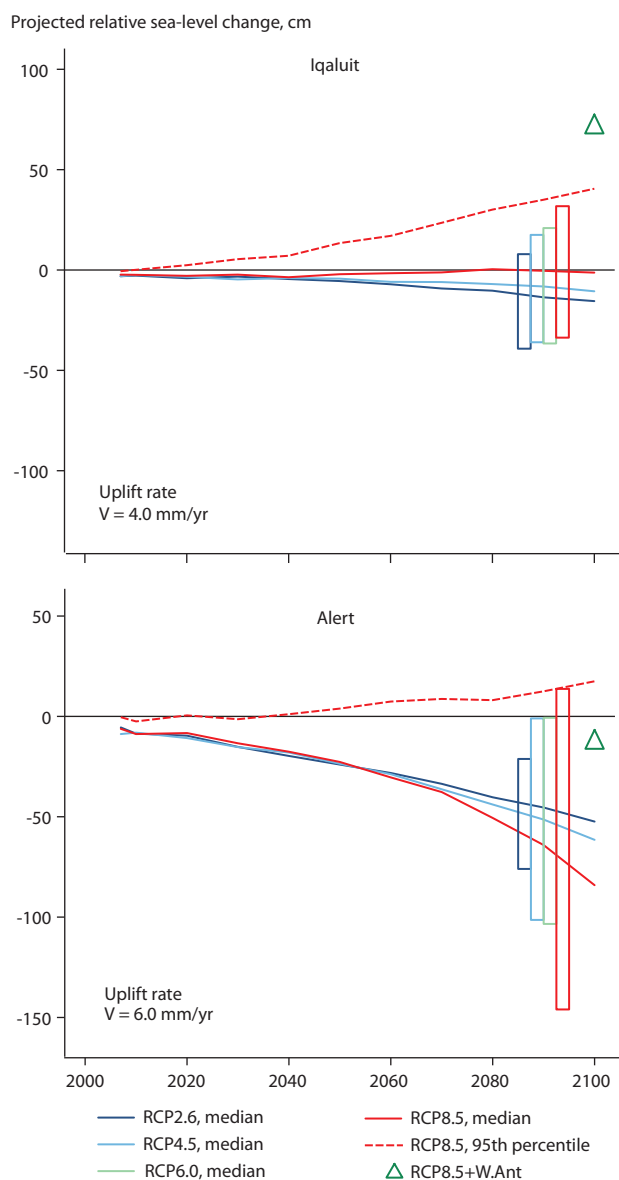
Figure 3.24 Projected relative sea-level change for Iqaluit and Alert (after James et al., 2014), based on the IPCC AR5 (Church et al., 2013a, 2013b) and also vertical crustal motion (uplift rate, given to nearest 0.5 mm/yr) derived from GPS observations. Projections are given through the century for the RCP2.6, RCP4.5, and RCP8.5 scenarios. The rectangles show the 90% confidence interval (5% to 95%) of the average projection for the period 2081–2100 for each of those three scenarios and also RCP6.0. The dashed red line gives the 95th percentile value for RCP8.5. The projected value at 2100 is also given for a scenario in which West Antarctica contributes an additional 65 cm of global sea level rise, added to the median projection of RCP8.5 (RCP8.5+W.Ant; green triangle).
