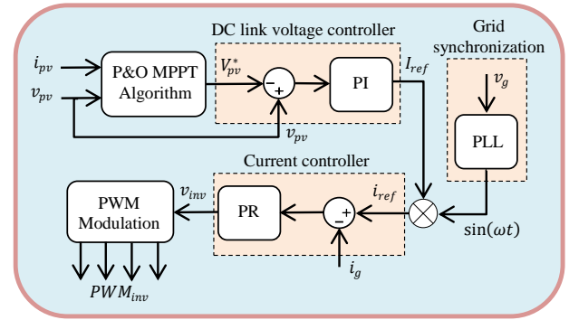
Fig. 2. Control structure for single-stage single-phase grid-connected PV inverter (PI - Proportional Integral, PR - Proportional Resonant, PWM - Pulse Width Modulation).
