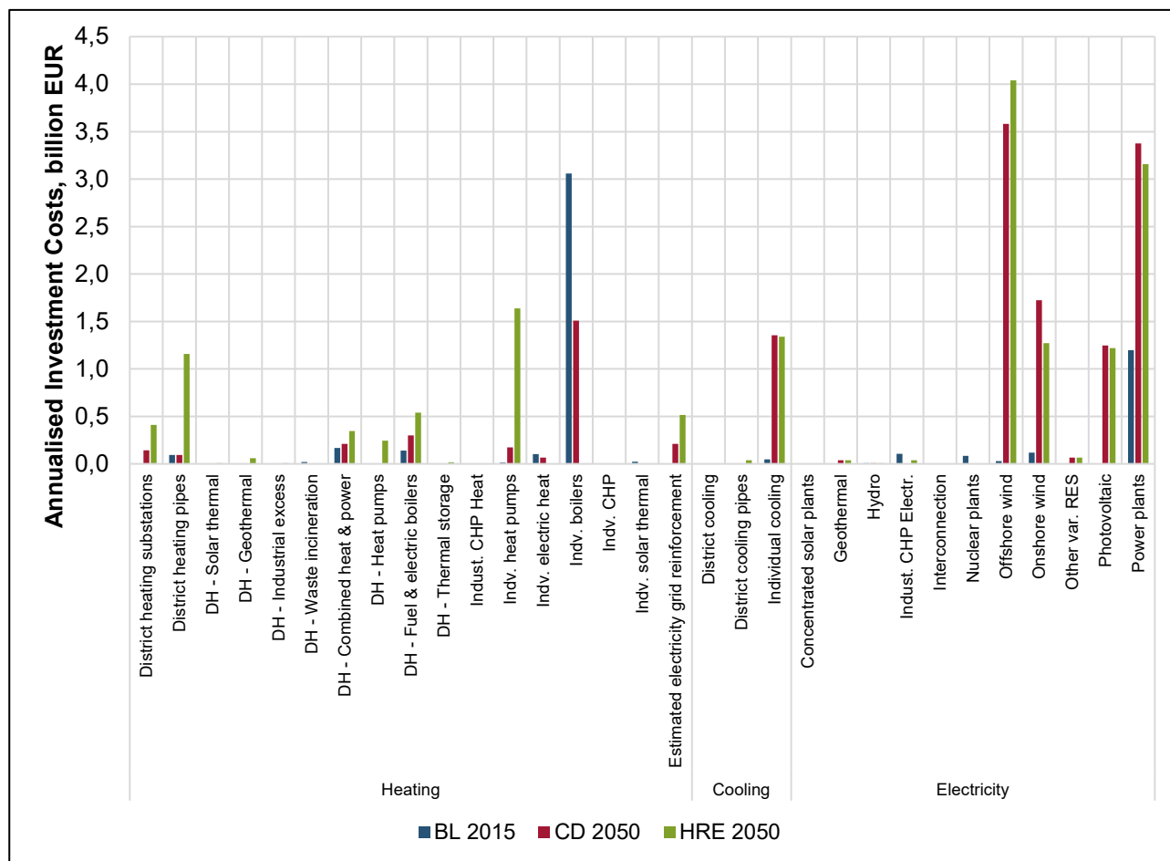
Figure 13. Annualised socio-economic investment costs and categories in the Netherlands, excluding the investment costs necessary for energy savings.
