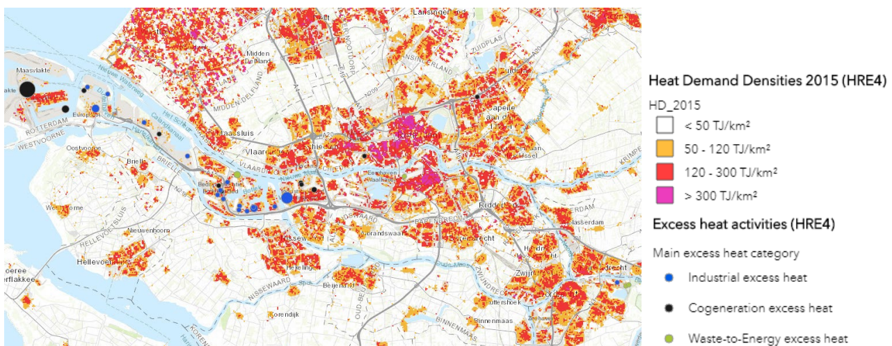
Figure 2. Heat demand density and excess heat activities Rotterdam.
