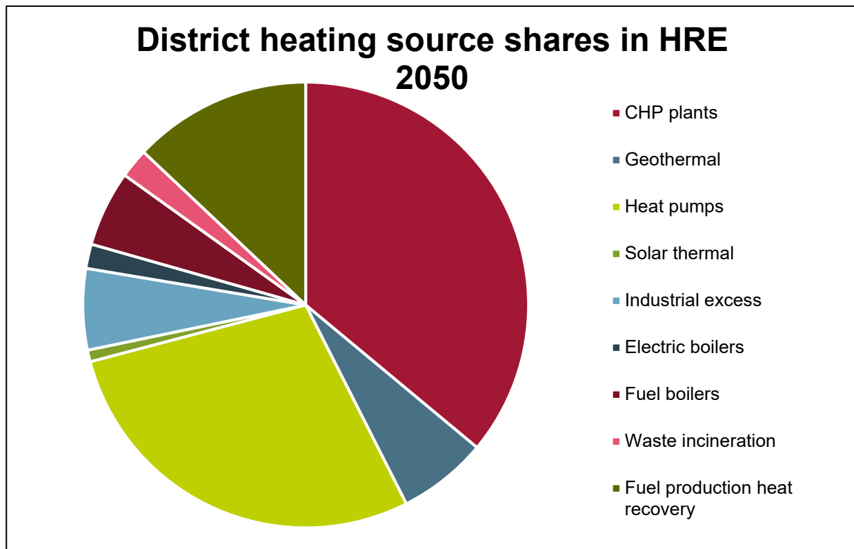
Figure 7. Heat sources for district heating in Heat Roadmap Netherlands.
