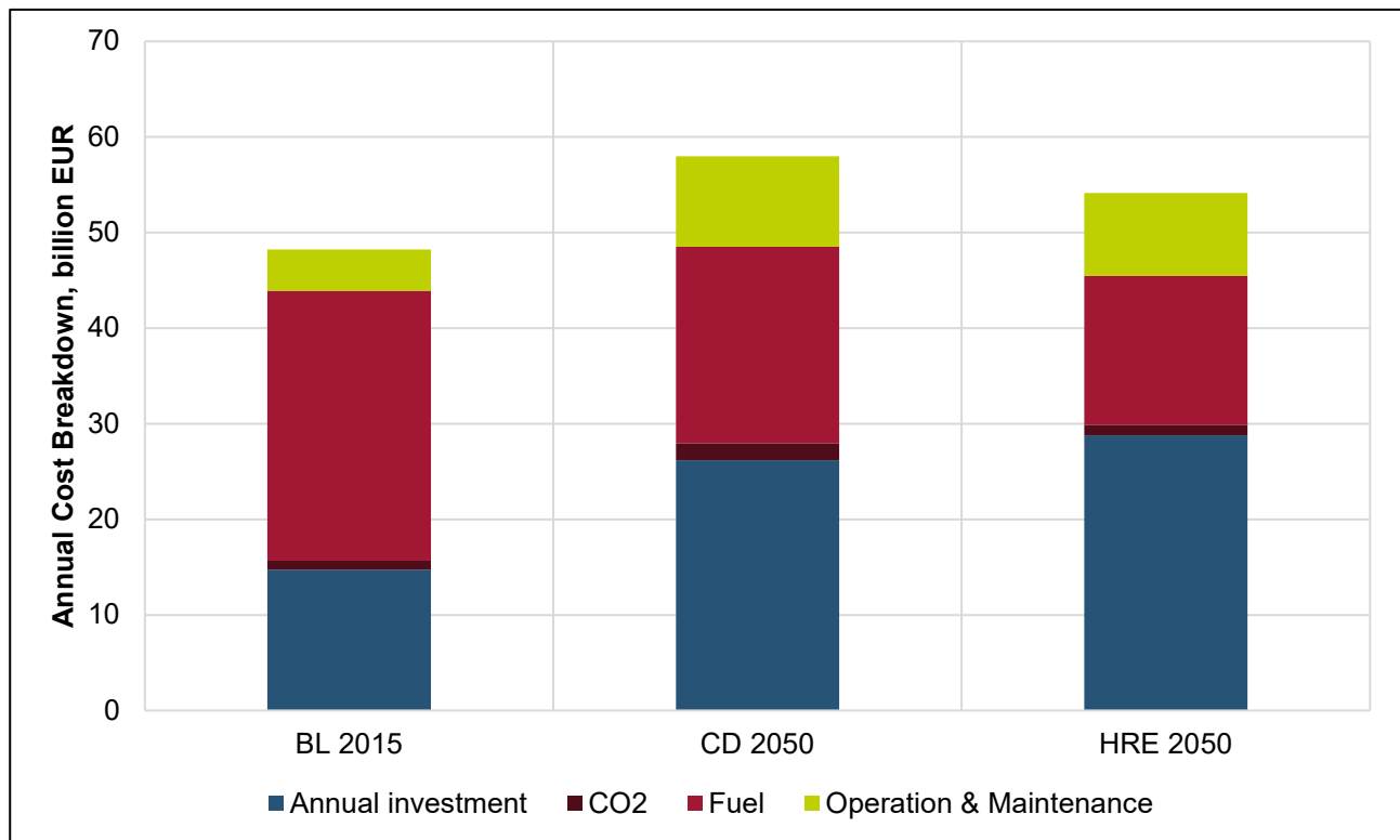
Figure 12. Annual socio-economic costs for the heating, cooling, electricity, industry, and transport sector for Netherlands.
