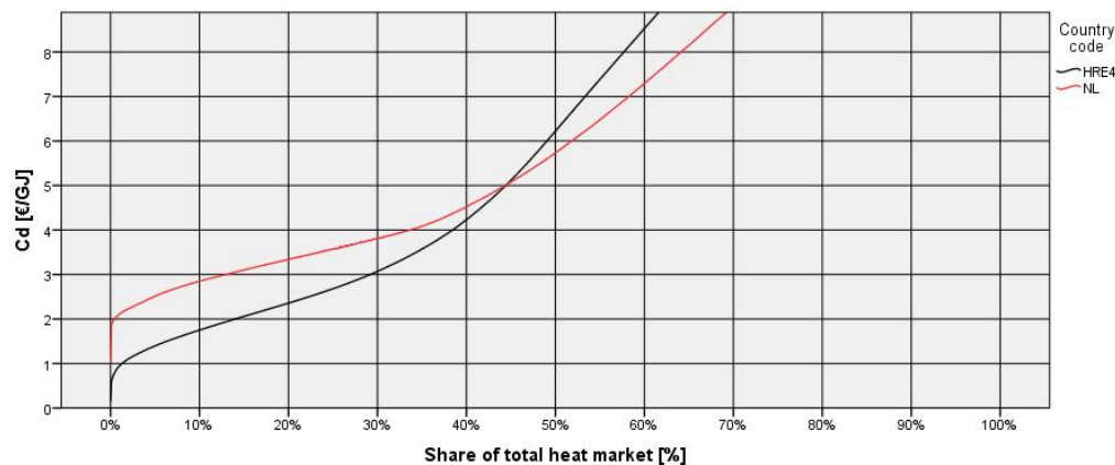
Figure 3. Distribution cost of heating at percentage share of total heat market for The Netherlands and HRE average.
