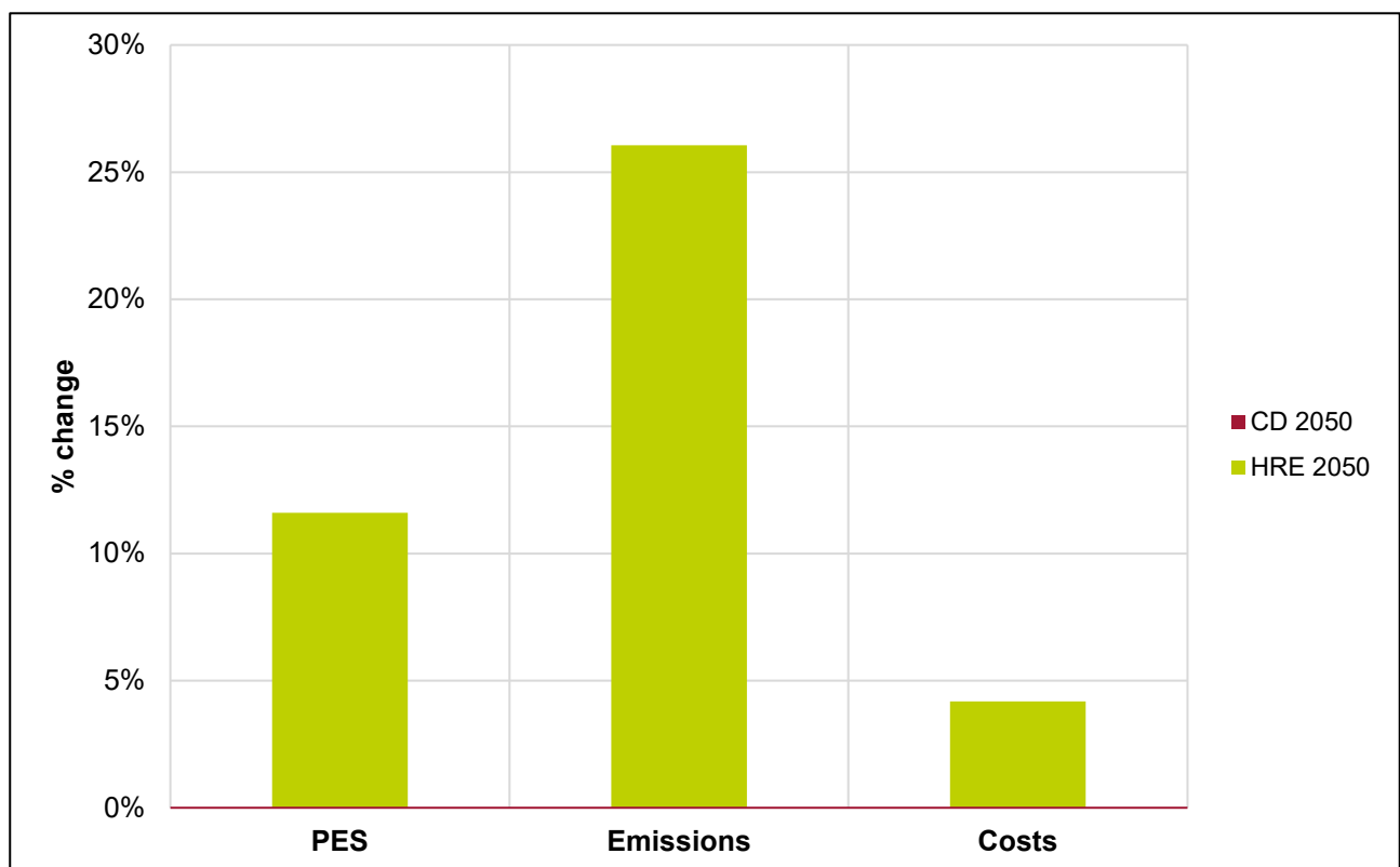
Figure 1. Percentage improvement in efficiency, energy and industry related emissions, and system costs of Heat Roadmap Poland (HRE 2050) compared to the conventionally decarbonized scenario (CD 2050).
