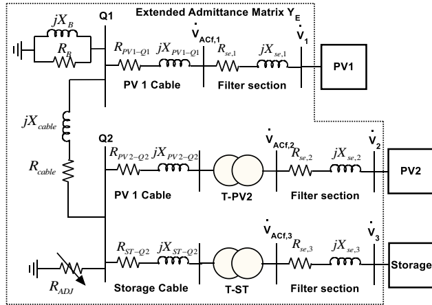
Fig. 6. SPM islanded section one-line diagram.
