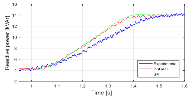
Fig. 12. Scenario B ST reactive power. Experimental data (blue line), PSCAD (red line) and SM (green line).
