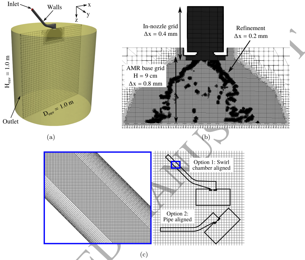
Figure 3: (a) The simulation domain consists of the nozzle and a cylindrical outside environment. (b) The different static and adaptive refinement regions with respective cell sizes. (c) The hexahedral part of the mesh can be aligned either with the swirl chamber and the outside environment or with the inlet pipe (Option 1 is used in the present work). The close-up shows a cross-section of the grid at the inlet pipe.
