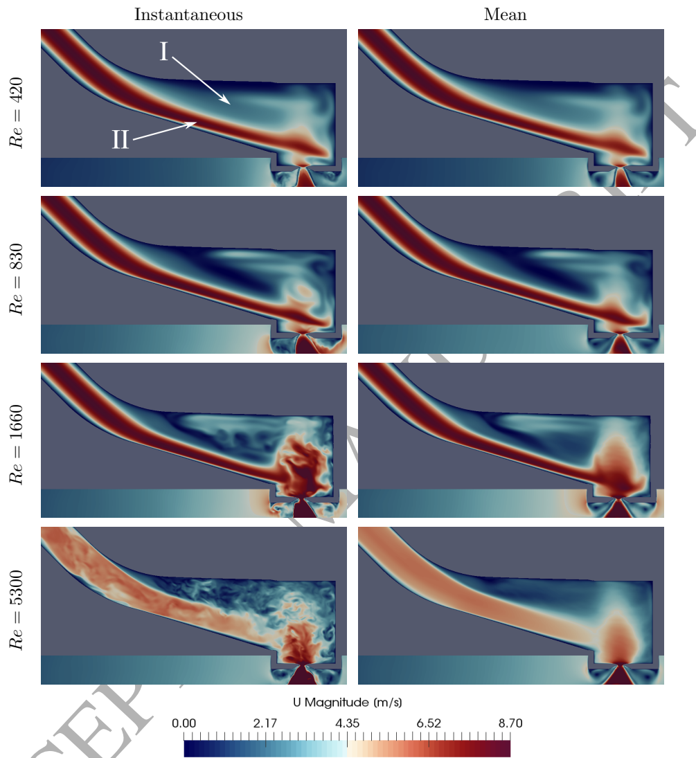
Figure 5: Instantaneous and mean velocity magnitude at the enlargement region and swirl chamber. The plane aligns with the axis of the inlet pipe and does not intersect with the air core inside the chamber.
