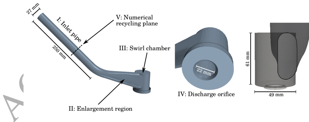
Figure 2: The nozzle geometry.
