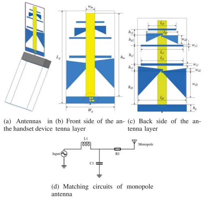
Fig. 1: Antenna configuration
