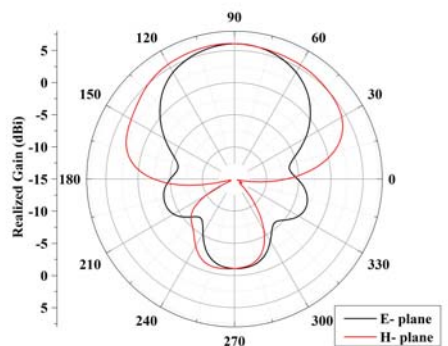
(c) E-plane and H-plane radiation pattern of L band antenna
