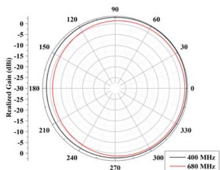
(b) H-plane radiation pattern of UHF antenna at 400 MHz and 680 MHz
