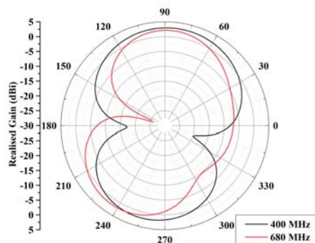
(a) E-plane radiation pattern of UHF antenna at 400 MHz and 680 MHz
