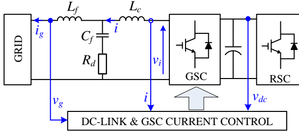
Fig. 3. Equivalent single-phase grid-side converter with LCL filter.
