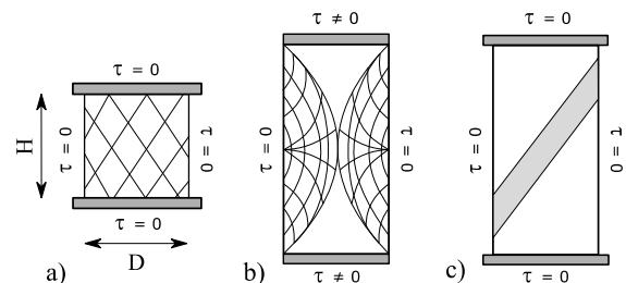
Fig 1. a) sample with smooth ends and H/D=1, b) tall samples with rough ends imply dead zones at the ends, c) tall samples and smooth ends cause a single line failure.
