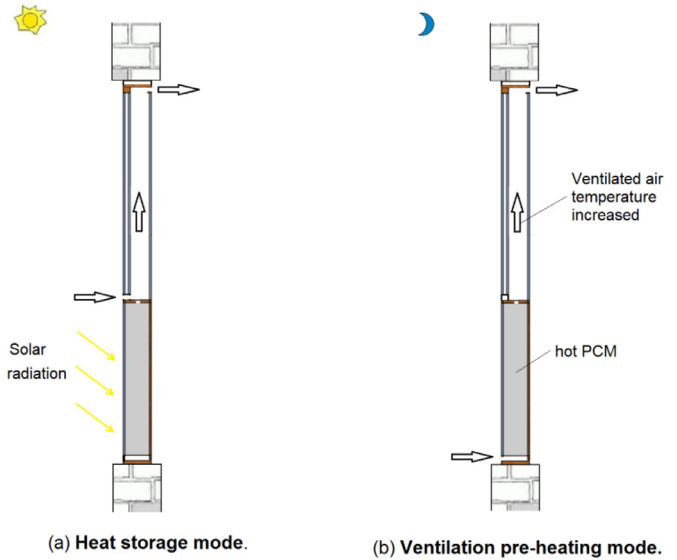
Fig. 4. Working principle of the PCMVV system in ventilation pre-heating application.
