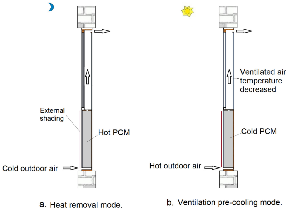
Fig. 3. Working principle of the PCMVV system in ventilation pre-cooling application.
