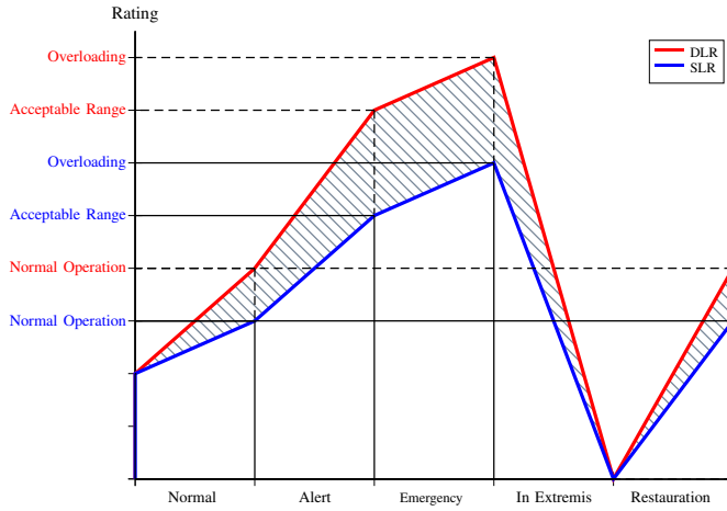
Figure 2. Influence of DLR in operating states of power systems
