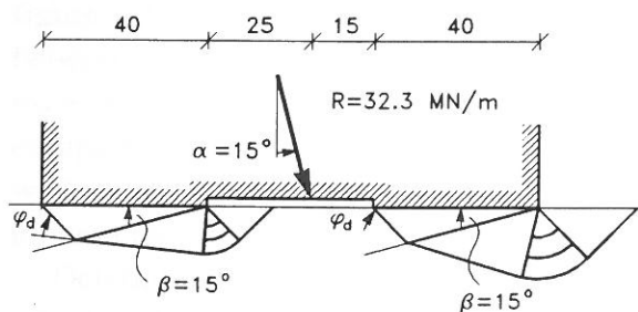
Fig. 9. Rupture figure, Upper Bound analysis
