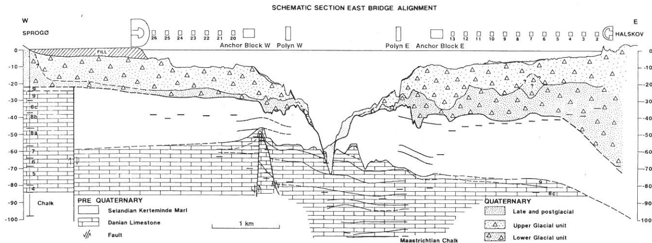
Fig. 4. Schematic geological section in East Bridge alignment (after Foged et al, 1995)
