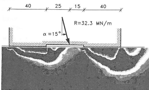
Fig. 10. Rupture figure, ABAQUS analysis
