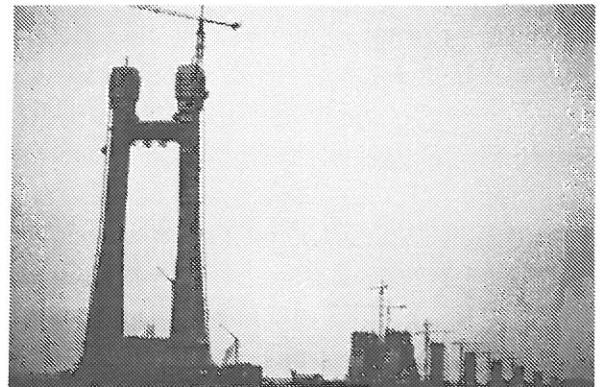
Fig. 12. Pylons, anchor blocks and approach piers of the East Bridge in early 1995 (Photos by S. Madsen)
