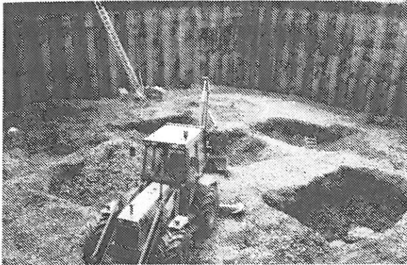
Fig. 11. Excavation of crushed stone in trial pit
