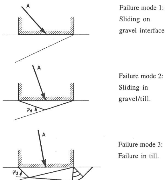
Fig. 8. Foundation Pad Failure Modes
