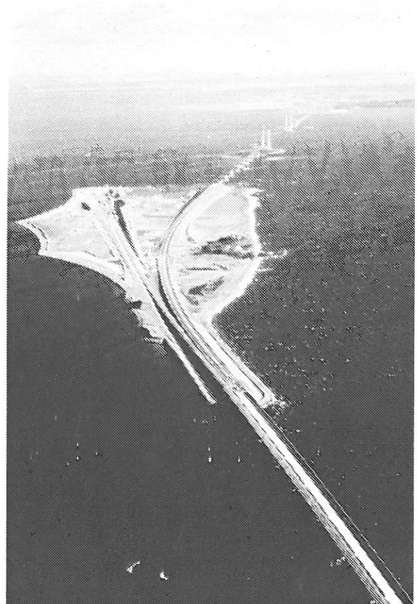
Fig. 1. Birds view of Storebælt Link project, Denmark in late 1994 (Photo by J.K. Winther)
