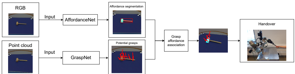
Figure 3: Proposed two-stage method for task-oriented grasping by combining affordance segmentation and task-agnostic grasp sampling.
