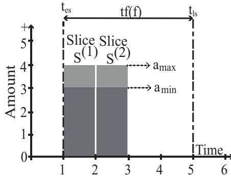
Fig. 1.1: Illustration of a flex-offer
