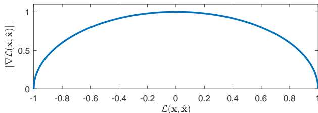
Fig. F.1: \ell^2 -norm of Eq. (F.5) as function of cost function value.
