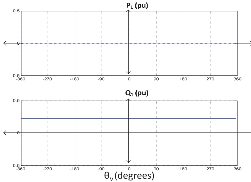
Fig. 3.4 Power -angle characteristics for V_1=0.3 pu, V_2=0 pu, and Z=j0.4 pu
