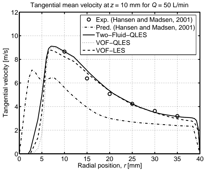
Figure 7.9: Mean tangential velocity profiles for flow rate of 50 L/min.
