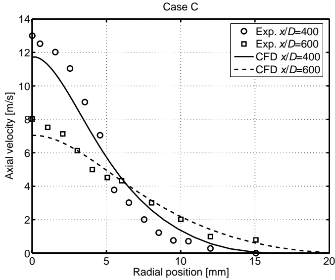
Figure 8.4: Axial liquid velocity for case C.
