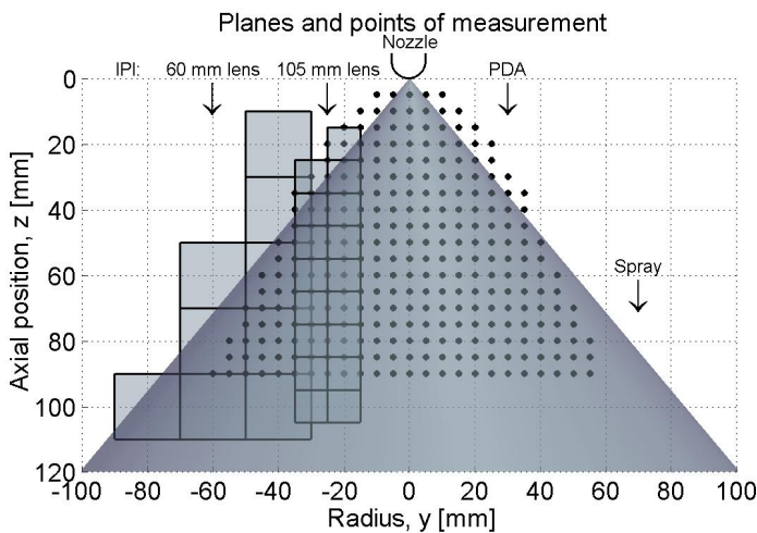
Figure 4.12: Location of IPI measuring planes and PDA measuring points.
