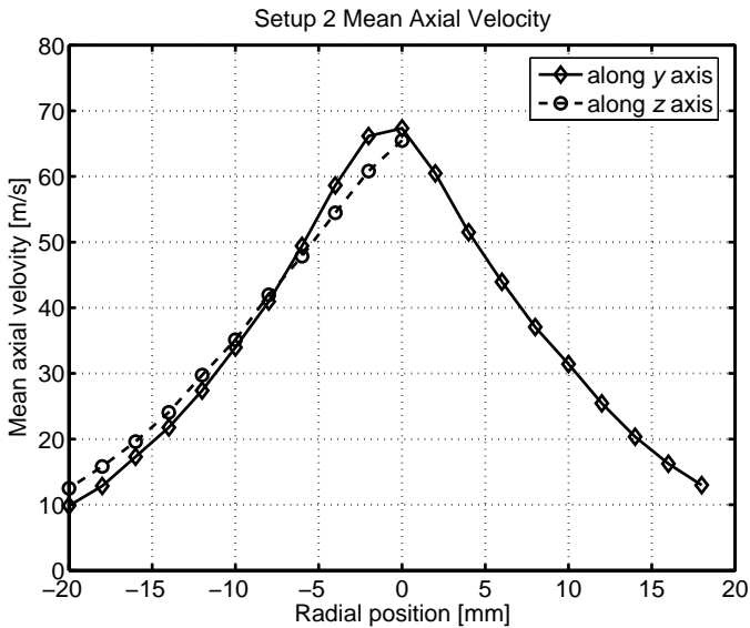
Figure 4.32: Distribution of droplet mean axial velocity along two orthogonal directions y and z at x = 150 mm in Setup 2.
