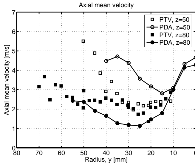
Figure 4.22: Comparison of mean axial velocity at different axial positions from PTV and PDA.
