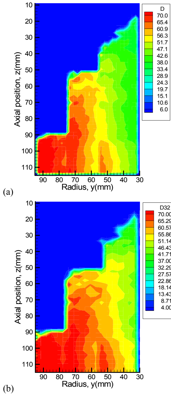
Figure 4.18: Ensemble averaged contour plot of (a) D_{10} and (b) D_{32} .
