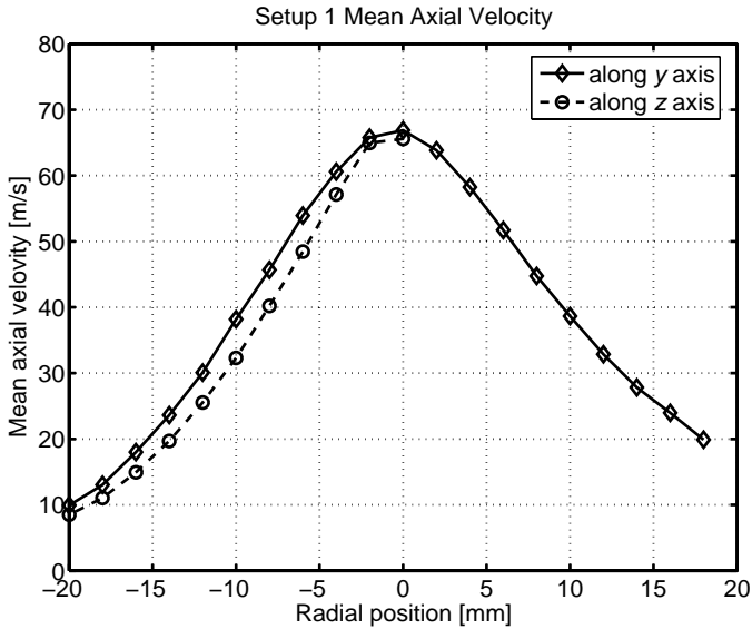
Figure 4.31: Distribution of droplet mean axial velocity along two orthogonal directions y and z at x = 150 mm in Setup 1.
