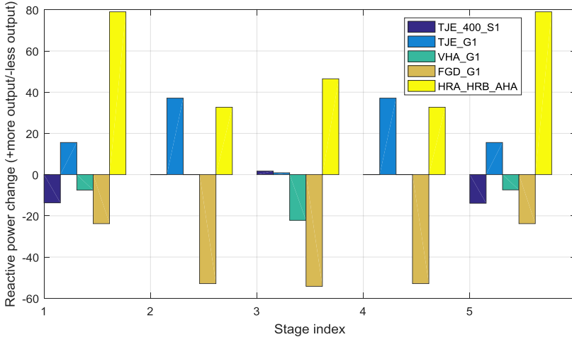
Figure 108. The change of the reactive power output for the continuous reactive power components in the critical scenarios, where wind farms participate in AVC. “AHA”: Anholt wind farm; “HRA” and “HRB”: Horns Rev A and B wind farm, respectively; “FGD_G1”, “VHA_G1” and “TJE_G1” are synchronous condensers; TJE_400_S1 is VSC-HVDC link. Positive means more reactive power output from the components after employing the wind farms and vice versa.
