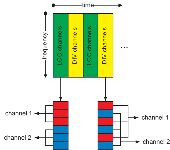
Figure 4.2: LOC and DIV subchannels within an OFDM frame
