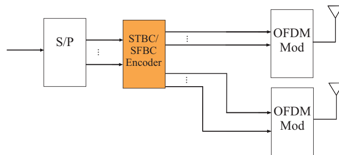
Figure 2.3: STBC and SFBC in OFDM
