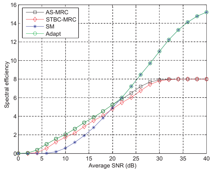
Figure 4.15: Spectral efficiency of MIMO 2 \times 2 look-up table with no delay
