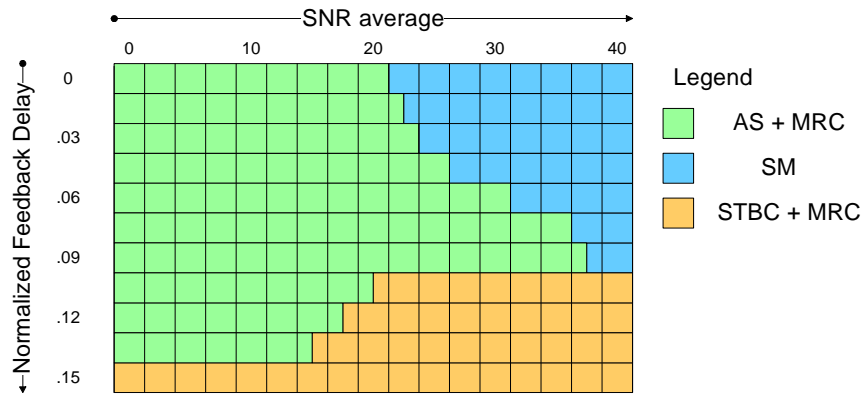
Figure 4.14: MIMO 2 \times 2 look-up table
