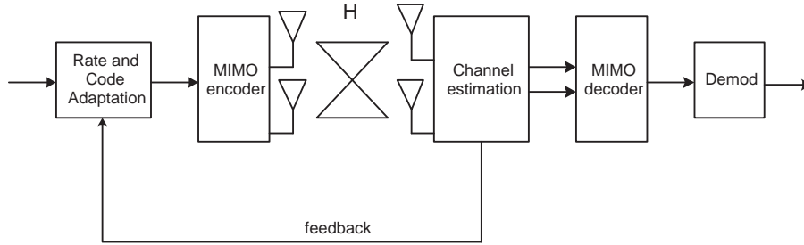
Figure 2.7: System model with MIMO and AMC
