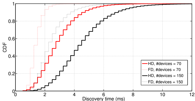
Fig. E.5: Multi-cluster. Cooperative maximum algorithm CDF
