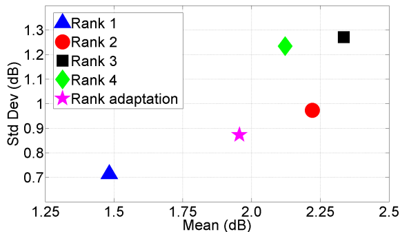
Fig. B.2: SINR variability ( \sigma_{SINR} ) characteristics
