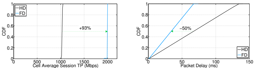
Fig. C.10: Bidirectional FD performance in a single cell network with 100% probability of exploiting FD.
