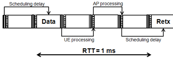
Fig. A.2: Round trip time for a downlink transmission
