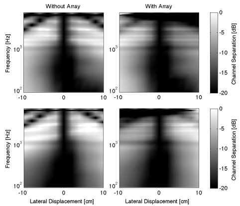
Fig. 8: Channel separation as function of frequency and lateral displacement single loudspeaker pair (left) and a loudspeaker array with super directive beamformer (right). Span angle 60^\circ
