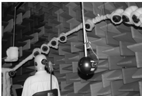
Fig. 10: Rotating loudspeaker.
