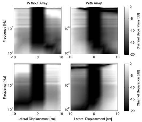
Fig. 7: Channel separation as function of frequency and lateral displacement single loudspeaker pair (left) and a loudspeaker array with super directive beamformer (right). Span angle 16^\circ
