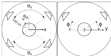
Fig. 2. General diagram of the measured loudspeaker configurations. \theta_s corresponds to the span angle and \phi corresponds to the elevation angle. Only the loudspeakers in front of the listener were used to evaluate the two-channels configuration.
