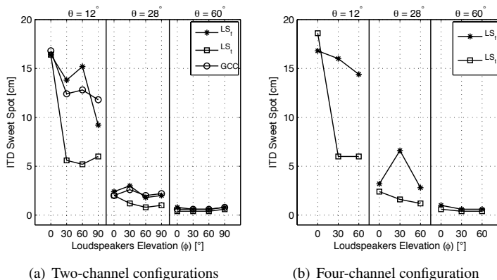
Fig. 3. ITD sweet spot size for lateral displacements as function of loudspeaker configuration. Each column corresponds to each measured span angle \theta_s , and the x-axis to each measured elevation \phi . Only the two-channel configuration was measured at 90^\circ elevation.
