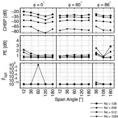
Fig. 10: Performance of the least square method in time domain at the left ear as a function of loudspeakers position applied to the two-channel configurations ( f_0 = 8 kHz). The values of the channel separation index (CHSP), the performance error index (PE) and the optimum regularization \beta_{opt} (see equation 18) are displayed.
