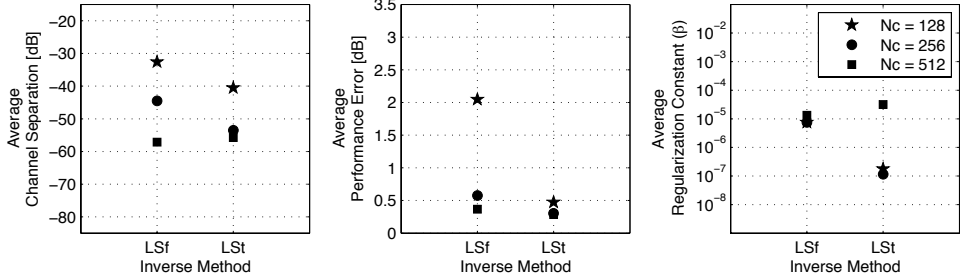
Fig. 13: Average over all symmetric loudspeaker arrangement evaluated at the left ear for the least square method in the frequency domain (LSf) and in the time domain (LSt) ( f_0 = 14 kHz)
