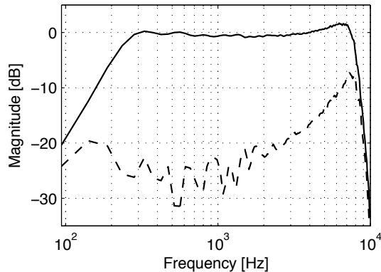
Figure 1.4: Frequency response of the direct signal (solid line) and crosstalk (dashed line) measured at the left ear of a dummy head. The loudspeaker configuration used is 12^\circ span angle placed above the mannequin’s head. The shape factor used is a band-stop filter with stop bands at 500 Hz and 6 kHz and the regularization constant is set to \beta = 0.0082 .
