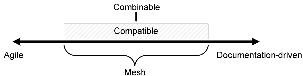
Figure 5. The mesh of agile and documentation-driven practice areas
