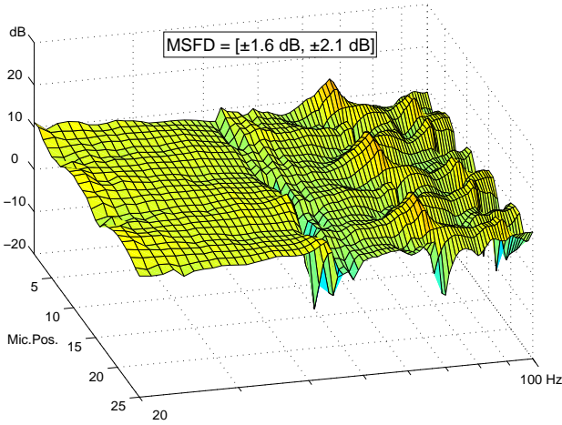
Fig. 46. Mean Sound Field Deviation ( MSFD ) of high pass filtered transfer functions at the listening area measured in the IEC Room. Upper setup .2.0. Lower after applying CABS .2.2. The loudspeaker response has been deconvolved.
