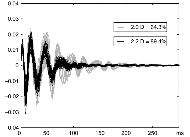
Fig. 43. The 25 impulse responses at the listening area resulting from measurements in the ITU Room and calculation of Definition D . Gray lines setup .2.0. Black lines after applying CABS .2.2 .
