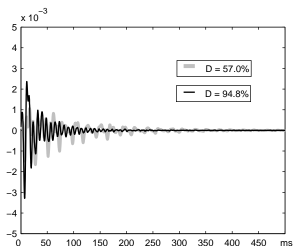
Fig. 23. Gray curve, impulse response of the listening position before equalization. Black curve the same position after the equalization resulting of simulations of Virtual Room, loudspeaker setup .2.0 .
