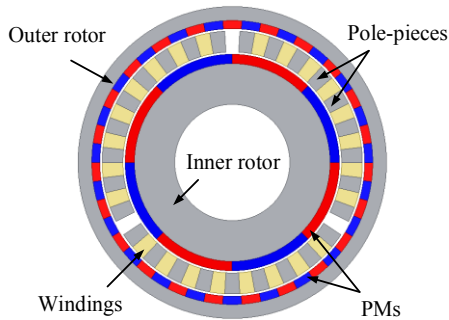
Figure 1-21 One two-air-gap MGM with sandwiched armature windings.
