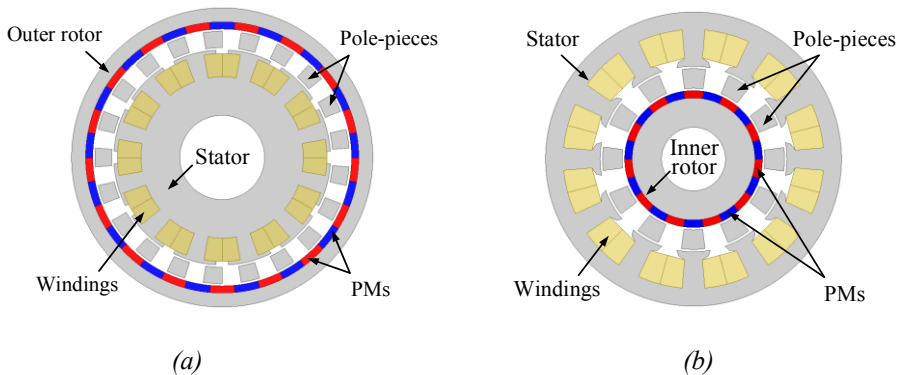
Figure 1-22 Two-air-gap MGMs with one PM ring, (a) with inner stator, (b) with outer stator.
