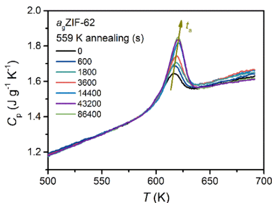
Figure 4-4 Temperature dependence of C_p of a_g\text{ZIF-62} annealed at 559 K for different durations t_a (in seconds).
