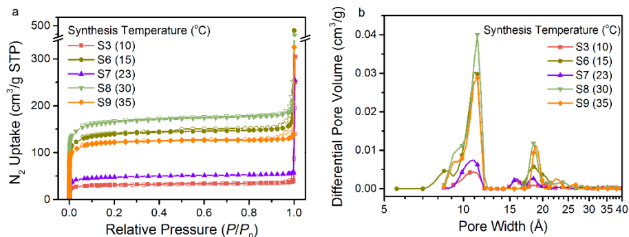
Figure 3-9 N_2 absorption-desorption isotherms of samples S3 and S6-S9 synthesized at different temperature. Solid and open symbols: Absorption and desorption, respectively. (b) Pore size distribution.
