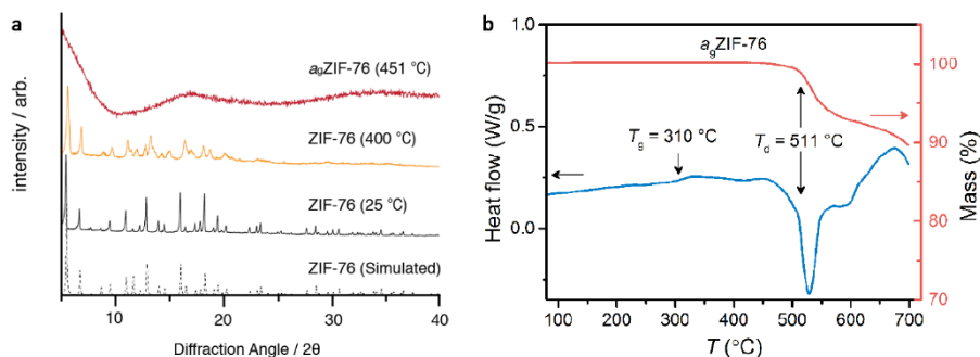
Figure 5-9 (a) PXRD patterns of the a_g ZIF-76 and ones preheated at 400 °C and melting point (451 °C). (b) DSC-TGA upscan curves of the a_g ZIF-76.
