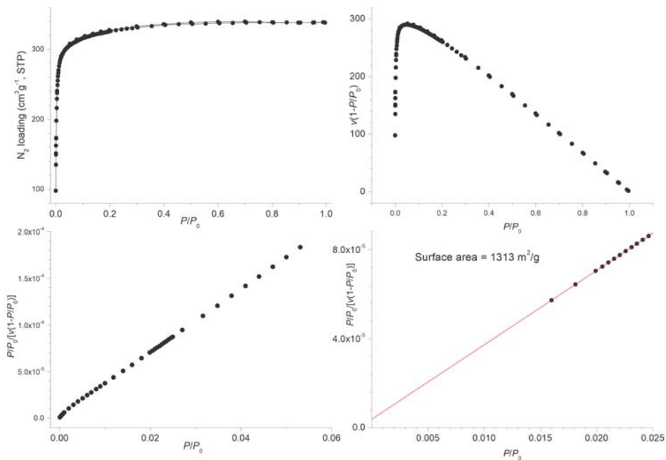
Supplementary Figure 23. N_2 adsorption isotherm at 77 K and BET surface area plots for ZIF-76, [Zn(Im)_{1.0}(5-ClIm)_{1.0}] .
