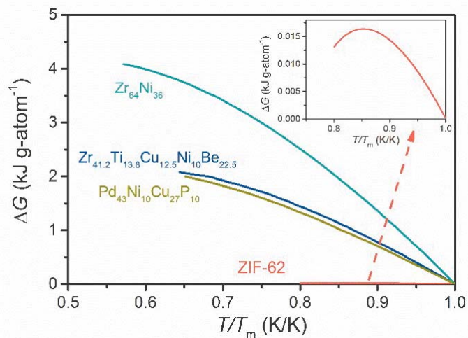
Fig. S2 Differences in the Gibbs free energy difference \Delta G^{sl-x}(T) between the supercooled liquid and the crystal of ZIF-62, using a \text{kJ g-atom}^{-1} basis (18.5 atoms per ZIF-62 molecule according to the formula). The \Delta G^{sl-x}(T) of some alloys are also given as comparisons from literature, in which one atom is taken as per mol.
