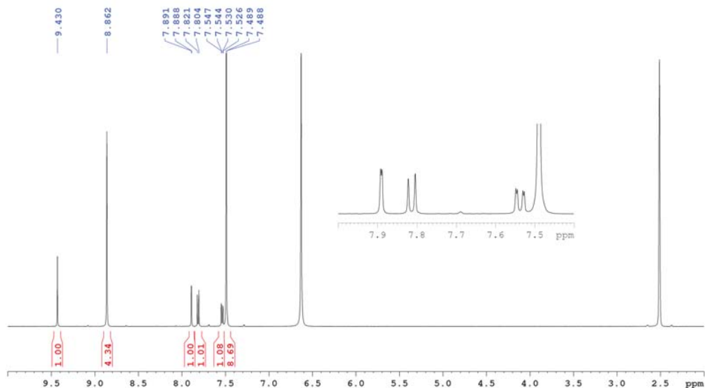
Supplementary Figure 5. ^1\text{H} NMR spectrum of a_9\text{ZIF-76} digested in DCI/DMSO- d_6 . NMR peak assignments: \text{Zn}(\text{Im})_{1.62}(\text{Ciblm})_{0.38} . ^1\text{H} NMR (500 MHz, DMSO- d_6 ): 2.5 (DMSO- d_6 ), 7.49 (CHCHN lm ), 7.55 (CCHCH Ciblm ), 7.81 (CCHCH Ciblm ), 7.89 (CICCHCC Ciblm ), 8.86 (NCHN lm ), 9.43 (NCHN Ciblm ).
