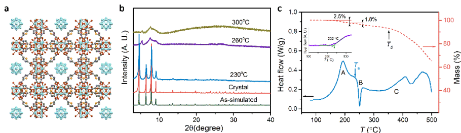
Figure 5-11 (a) Unit cell of DUT-67 from the direction of b axis. Gray: C; Yellow: S; Red: O; Light blue: Zr. H atoms are omitted for clarity. (b) PXRD patterns of the as-synthesized and simulated DUT-67, and ones heat-treated at 230 °C, 260 °C and 300 °C in argon. (c) DSC-TGA upscan curves of the as-synthesized DUT-67. Inset: DSC upscan after preheated at 260 °C.
