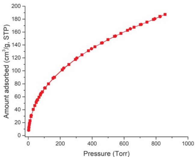
Supplementary Figure 24. H_2 adsorption isotherm at 77 K for ZIF-76, [Zn(Im)_{1.0}(5-ClIm)_{1.0}] (circles = adsorption; squares = desorption).
