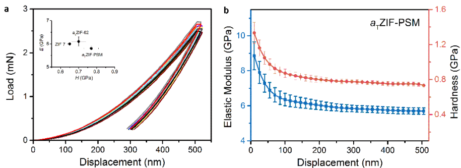
Figure 7-11 (a) Load-displacement curve from nanoindentation measurement of the a_T ZIF-PSM. Inset: E-H relationship of ZIF-7, a_T ZIF-62 and a_T ZIF-PSM (10,57). (b) Elastic modulus (E) and hardness (H) as a function of indentation depth of a_T ZIF-PSM. Error bars come from the standard deviation of 26 measurements.
