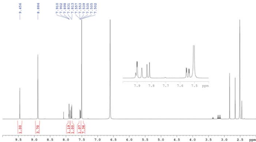
Supplementary Figure 2. 1 H NMR spectrum of as-synthesized ZIF-76 digested in DCI/DMSO-d 6 . NMR peak assignments: Zn(Im) 1.62 (ClbIm) 0.38 . 1 H NMR (500 MHz, DMSO-d 6 ): 2.5 (DMSO-d 6 ), 7.50 (CHCHN Im ), 7.54 (CCHCH ClbIm ), 7.82 (CCHCH ClbIm ), 7.90 (CICCHCC ClbIm ), 8.89 (NCHN Im ), 9.46 (NCHN ClbIm ).
