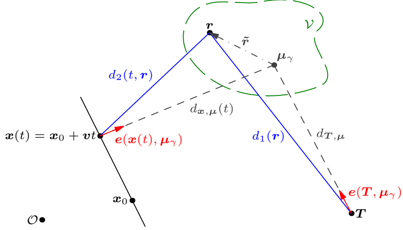
Fig. D.1: Generic LMS scenario with a mobile receiver moving nearby a single scattering volume \mathcal{V} : the transmitter is located at position \mathbf{T} , the receiver moves at constant velocity along the straight trajectory \mathbf{x}(t) . In the figure, \mathcal{O} denotes the origin of the coordinate system, \mathbf{r} is the position of a point-source scatterer in the volume, while \mathbf{x}_0 and \mathbf{v} denote respectively the position at t = 0 and the velocity of the receiver. The figure also includes the quantities that appear in the approximations of d_1(\mathbf{r}) and d_2(t, \mathbf{r}) introduced in the sequel (see (D.24) and (D.25)).
