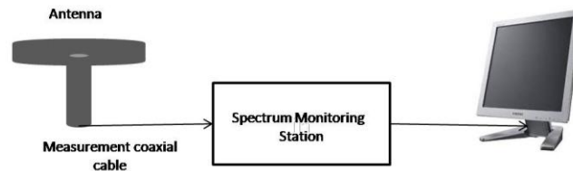
Figure 2.3: Measurement Configuration
