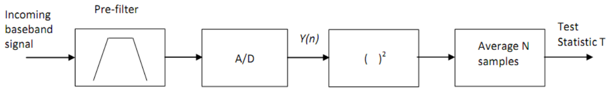
Figure 2.1: Conventional Implementation of Energy Detector [36]
