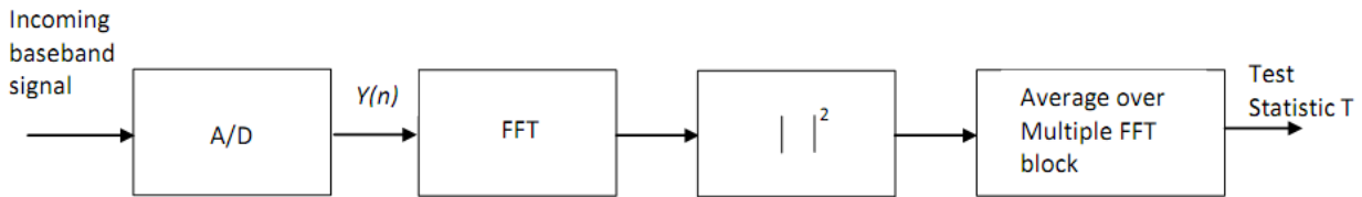
Figure 2.2: Implementation of Energy Detector Using Periodogram [36]
