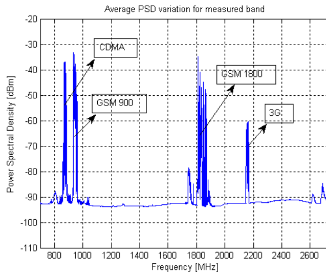
Figure 5.1: Average PSD Variation over Frequency Range 700-2746.6 MHz [98]
