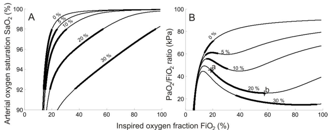
Figure 9: Simulated variation in \text{SaO}_2 (A) and \text{PaO}_2/\text{FiO}_2 ratio (B) upon changing \text{FiO}_2 under varying levels of shunt ( f_s ). Thick solid lines indicate the portion of the curves within the clinically relevant range of \text{FiO}_2 . a and b in subplot B indicate a variation in \text{FiO}_2 from 0.19 to 0.57 for f_s=20\% . Simulations were performed using \Delta\text{P}\text{O}_2 = 0 \text{ kPa} ( fA_2=0.9 ), \text{VO}_2 = 0.26 \text{ l/min} , alveolar minute volume = 5.25 \text{ l} . Used with permission from paper I.
