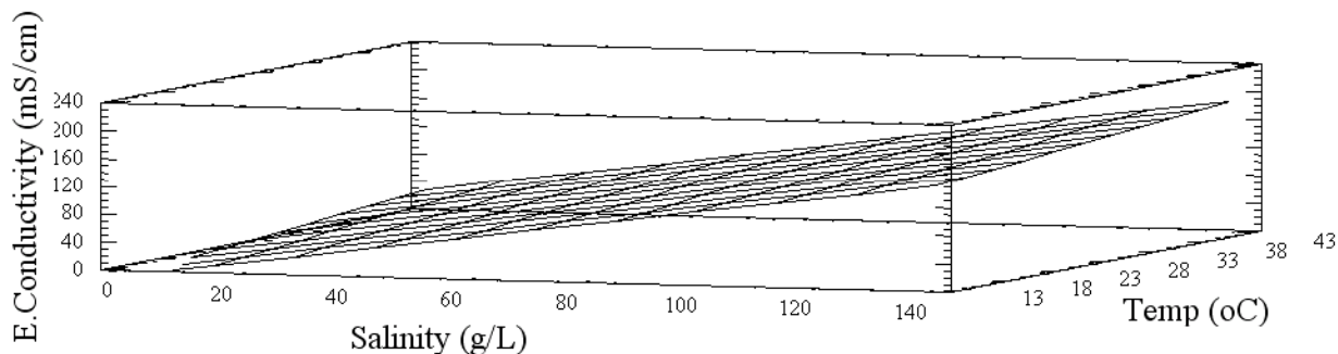
Fig. 11. Surface plot for electrical conductivity with salinity and temperature (Water A).
