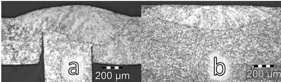
Figure 13 a) A weld performed with the three spot DOE as a double butt joint. Total power 400 W. and travel speed 50 mm/s.
