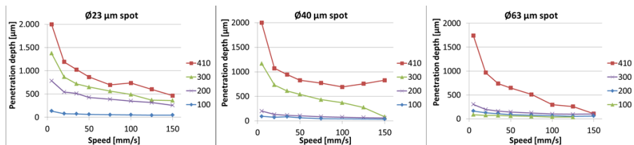
Figure 9 Comparison of penetration depth in stainless steel for different values of travel speed, laser power and spot size.
