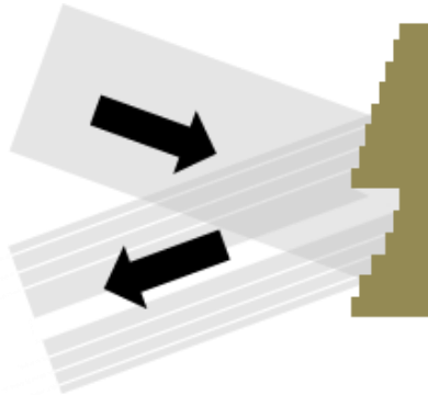
Figure 9 Cross section of a DOE. Example of shadow effect on the outgoing reflection of the laser beam for a reflective DOE. Dimension is out of scale, ratio between depth and width \gg 1 .
