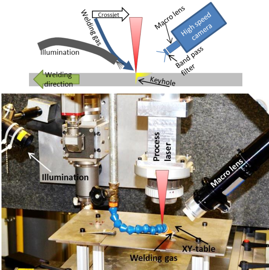
Figure 26 Setup for high speed photographing. Top) Principle. Bottom) Actual setup.
