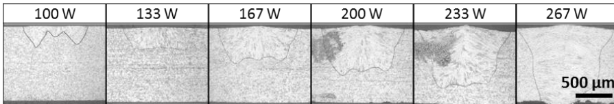
Figure 39 Cross-sections for different laser power performed as bead on sheet, all with focus placed on top of the sheet. (F0). Distances are a = 300 \mu\text{m} in all cases. Powers are average power per spot in the pattern. The applied pattern is the same as the one shown for the three spot patterns with a = 300 \mu\text{m} spacing in figure 36. All figures have the same scale.
