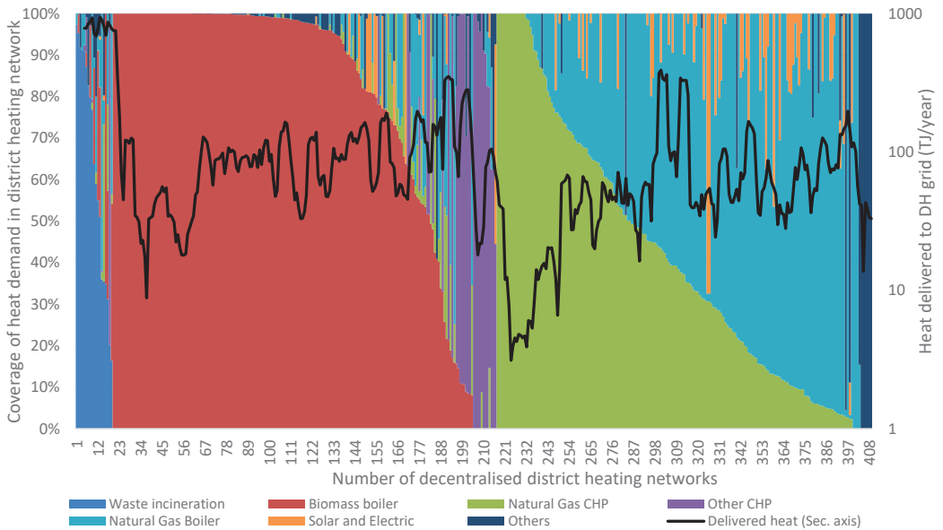
Figure 3 Diagram showing how decentralised DH plants cover their heat demands, sorted according to share covered by the different technologies. Delivered heat in each DH network is indicated by the black line (five-period average), referring to the secondary axis.
