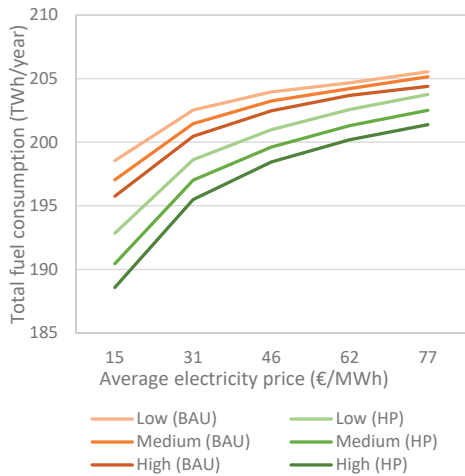
Figure 4 Energy market sensitivity analysis of fuel consumption. Low, Medium and High refer to the fuel price levels. BAU is the Business-as-usual scenario and HP shows implementation of 450 MW e of heat pump capacity (Moderate scenario).
