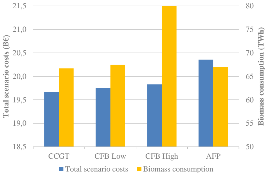
Figure 10: Main results for the scenarios of the technical energy systems analysis showing values for the whole energy system [2].
