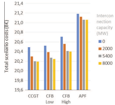
Fig. 8. Total costs for the scenarios of varying IC capacities without economic constraint on biomass consumption for fuel boilers in DH.
