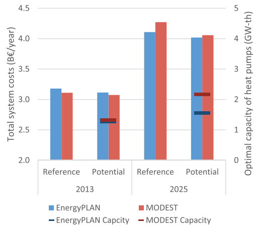
Fig. 5. Results of a closed system analysis (excluding electricity exchange) for the two scenarios, 2013 and 2025, showing the optimal heat pump capacities in the calculation of the heat pump potential. Line markers indicate optimal capacity of heat pumps.
