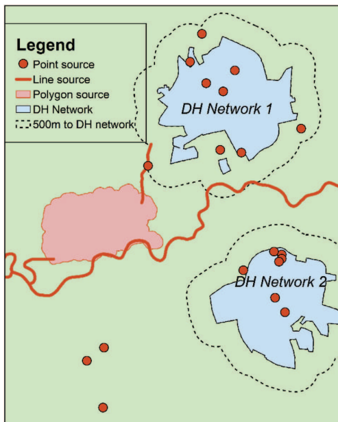
Fig. 2. Illustration of the mapping method. All heat sources that are within or intersect the dotted 500 m distance line are counted as potential heat sources.
