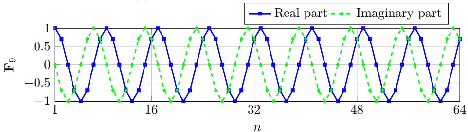
(b) 9th DFT basis vector.
