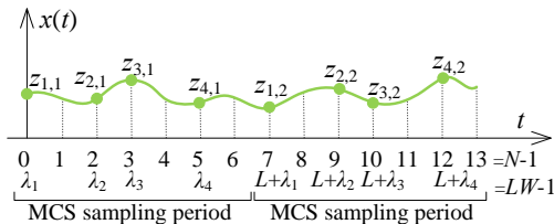
(b) MCS acquisition, L = 7 , W = 2 , P = 4 , \Lambda_{\text{MCS}} = \{0, 2, 3, 5\} .
