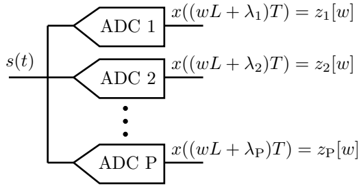
(a) Simplified MCS diagram.
