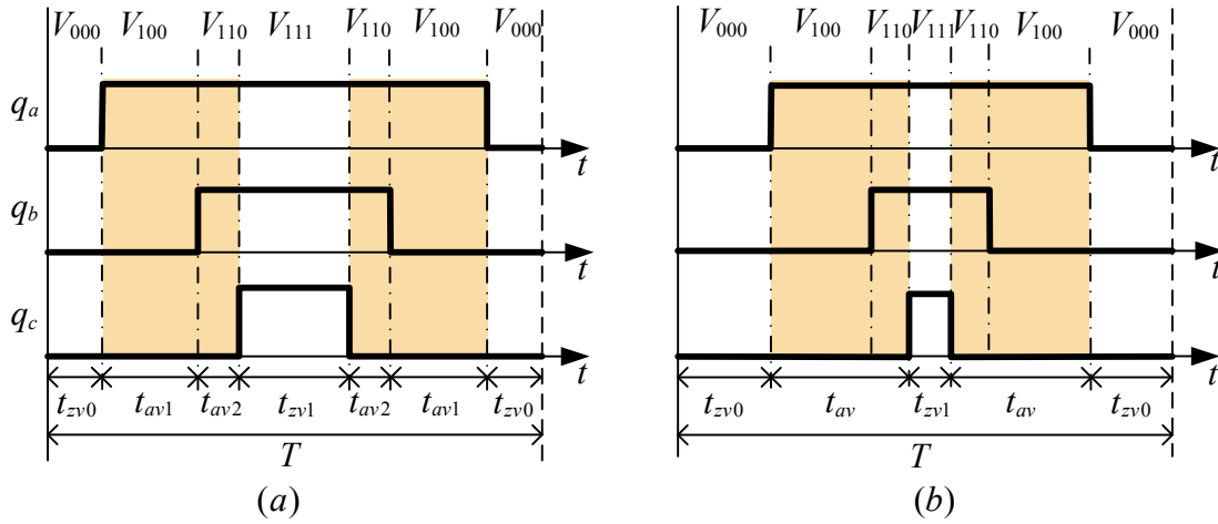
Figure 4-7 Pulse placement during a modulation period when t_{zv0}=t_{zv1} (a), and repositioning of the PWM pulses (b)
