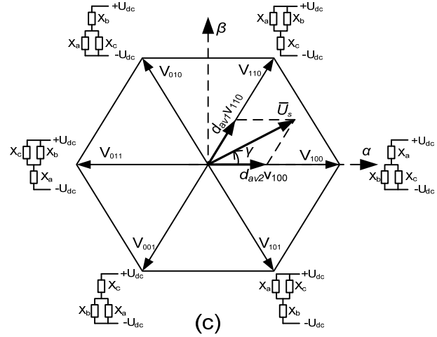
Fig. 1 Three-phase voltage-source converter (a) Circuit diagram, (b) Switching function during one period of the carrier (c) Space vector diagram in \alpha - \beta plane
