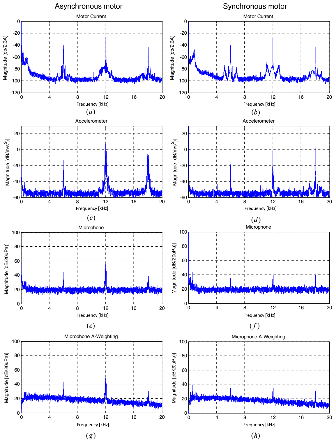
Figure 6-19 Measured spectrum of the motor current, vibration and acoustic noise at 150RPM on the asynchronous motor (left column) and synchronous motor (right column)
