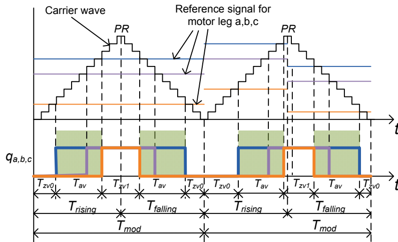
Figure 4-12 Digital implementation of RPP-PWM
