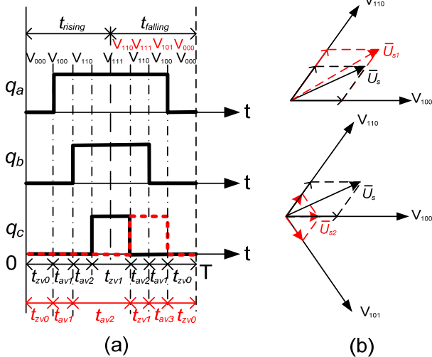
Fig. 2 Reposition of the pulse position in one leg. (a) pulses generated by symmetrical modulation (full line), changed position of the pulse on leg c (broken line), (b) vector diagram of the generated voltage vectors in the top first part of the modulation, in the bottom second part of modulation
