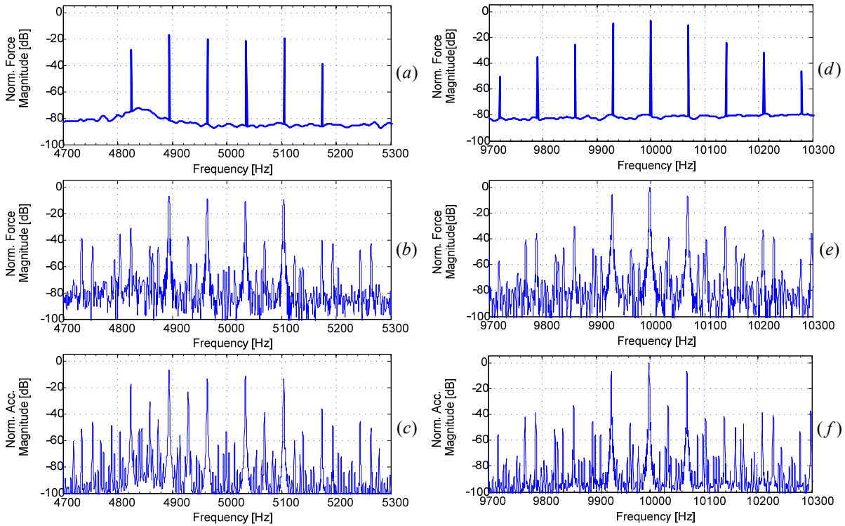
Figure 3-10 Zoom in vibration spectra of the coil: analytically calculated spectra at 5 kHz (a), vibration spectra using force look-up table at 5kHz (b), measured vibration spectra at 5kHz (c), analytically calculated spectra at 10kHz (d), vibration spectra using force look-up table at 10kHz (e), and measured vibration spectra at 10kHz (f)
