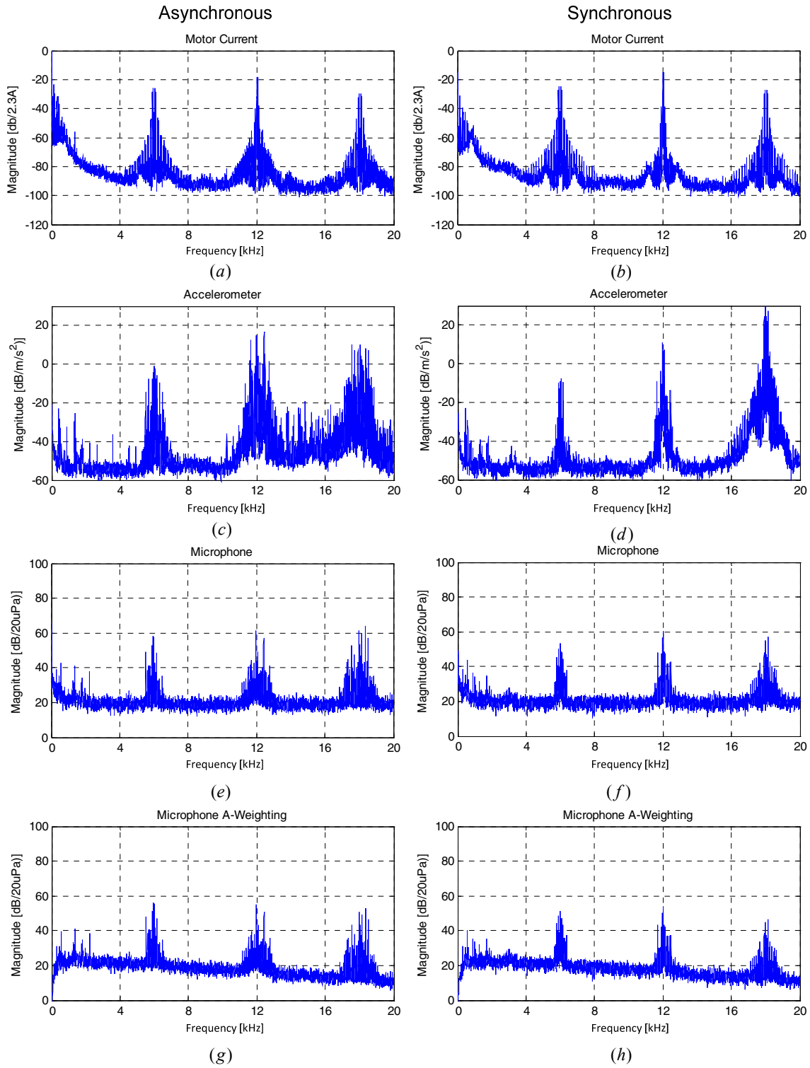
Figure 6-20 Measured spectrum of the motor current, vibration and acoustic noise at 750RPM on the asynchronous motor (left column) and synchronous motor (right column)
