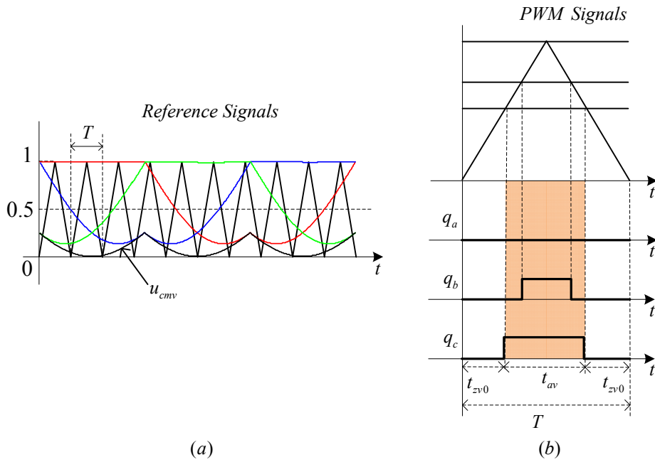
Figure 2-9 120^\circ Discontinuous PWM: reference signal waveforms (a), and pulse generation mechanism (b)
