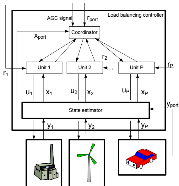
Figure 10.4: Sketch of the modular structure of the load balancing controller. Communication with the individual effectuator is handled by the independent subsystems, and portfolio communication is handled on the upper layer of the hierarchy. r_i is the reference to effectuator i \in \{1, 2, \dots, P\} , x_i is the state estimate, y_i is the measured output, and u_i is the controller correction. For the portfolio there is a reference r_{port} , state estimate x_{port} and a total measured production y_{port} . The references come from the production planning.
