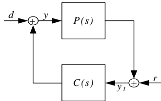
Figure 5.3: Block diagram used to check internal stability
