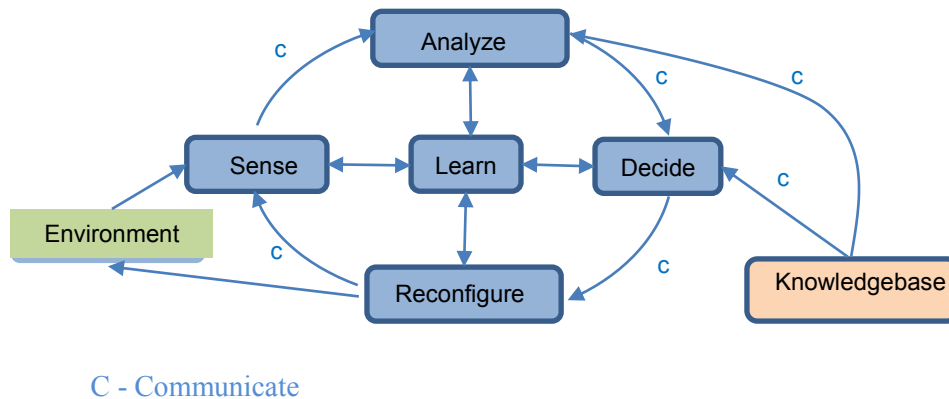
Figure 2-2 Enhanced Cognitive Meta Process
