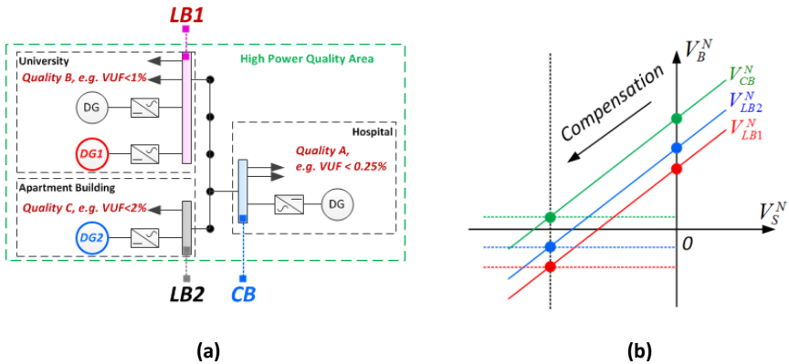
Figure 1.7. Voltage unbalance compensation in a multi-bus microgrid.
