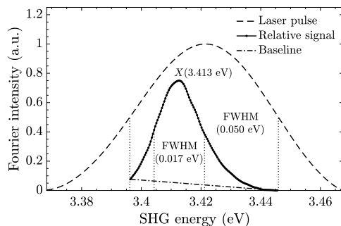
Fig. 5. The relative SHG Fourier intensity of the ZnO and quartz wedge samples measured with 10 nm FWHM laser pulses centered at 725 \pm 0.5 nm.
