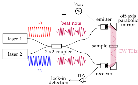
Fig. 1.3: Illustration of a typical CW THz spectrometer based on photomixers.
