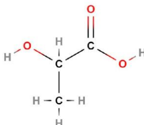
Figure 3. Structure of Lactic Acid ( C_3H_6O_3 ).
