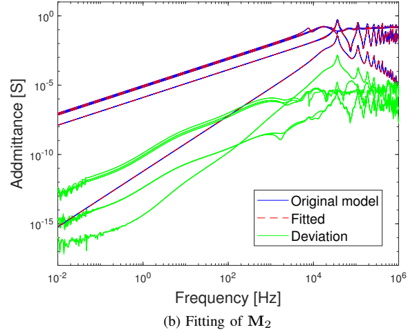
Fig. 6. Case #1: Fitting results (HVDC submarine cable)
