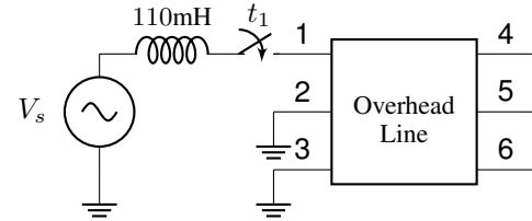
Fig. 12. Case #1: Circuit for time-domain simulation
