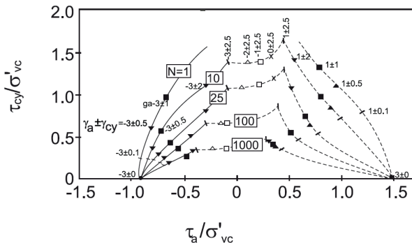
Figure 16: Number of cycles to failure, depending on cyclic and average load ratio. (Andersen and Berre, 1999)
