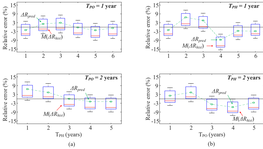
Fig. 3.8: Forecasting accuracy of the proposed forecasting method with relative error in the lifetime consumption of power converter based on the predicted environmental conditions \Delta R_{pred} and historical profiles \Delta R_{hist} (shown as a box plot) for varying: (a) Prediction horizons T_{PH} , and (b) Prediction offsets T_{PO} . Source: [J2].
