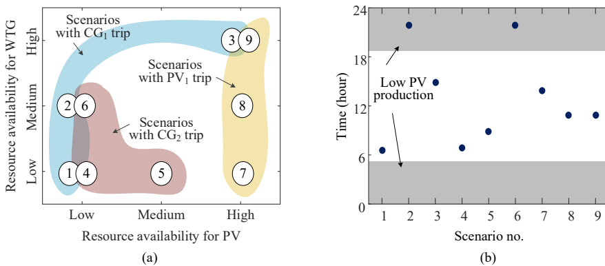
Fig. 5.7: Scenarios which lead to load shedding conditions in the power system: (a) Resource availability levels for CG 1 failures (marked in blue), CG 2 outages (marked in red) and PV 1 outages (marked in yellow), (b) Temporal characteristics in terms of time during the day that the scheduling data corresponding to the scenarios belongs to. Source: [J4].
