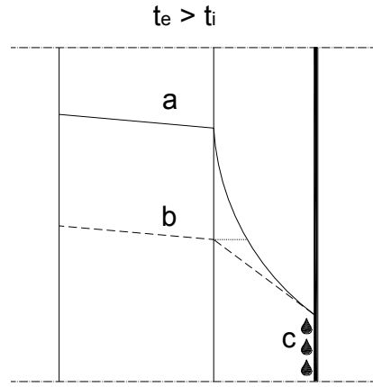
Fig. 1d. Vapour pressure distribution, sun. a. Saturated vapour pressure b. Actual vapour pressure c. Condensation
