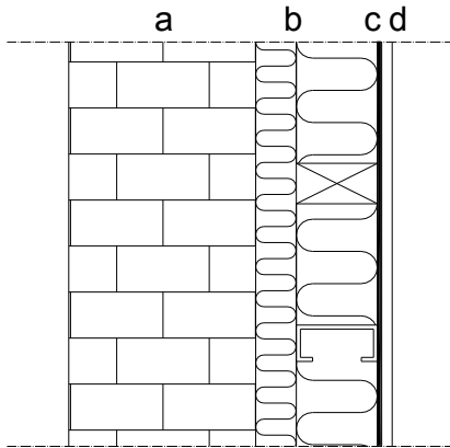
Fig. 1a. Interior insulated brick wall. a. Solid brick wall b. Insulated stud wall (or insulating panel) c. Vapour barrier d. 13 mm gypsum board
