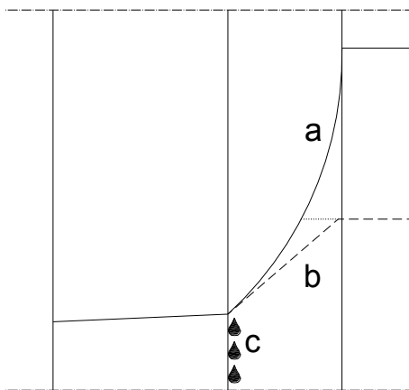
Fig. 1c. Vapour pressure distribution, air leakage a. Saturated vapour pressure b. Actual vapour pressure c. Interstitial condensation
