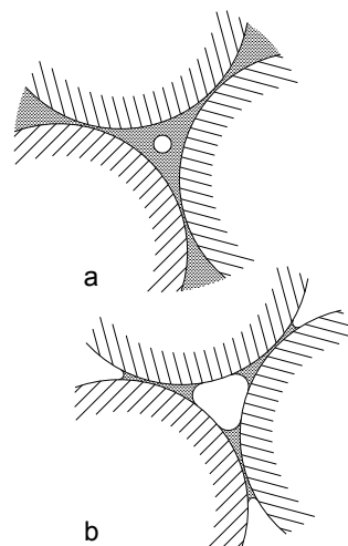
Fig. 2. Critical moisture content. a. Menisci filled, moisture transport possible b. Menisci not filled, moisture transport not possible
