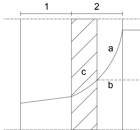
Fig. 1e. Zone with critical moisture content. 1. Solid brick wall 2. Calcium silicate boards a. Saturated vapour pressure b. Actual vapour pressure c. Area with critical moisture content
