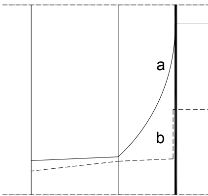
Fig. 1b. Vapour pressure distribution, PE-foil. a. Saturated vapour pressure b. Actual vapour pressure (no interstitial condensation)
